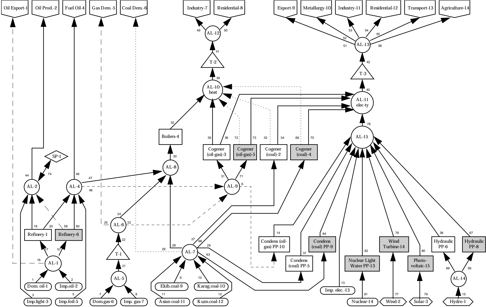
Figure 2. Kazakstan Energy Network
