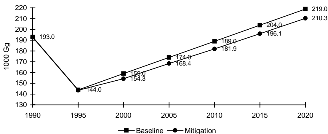
Figure 10. CO 2 Emissions Projections for Baseline and Mitigation Scenarios According to the Expert Judgments
