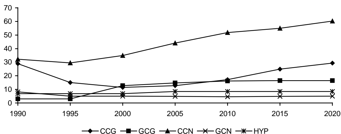
Figure 11. Electricity Generation under the Baseline Scenario (million kWh)
